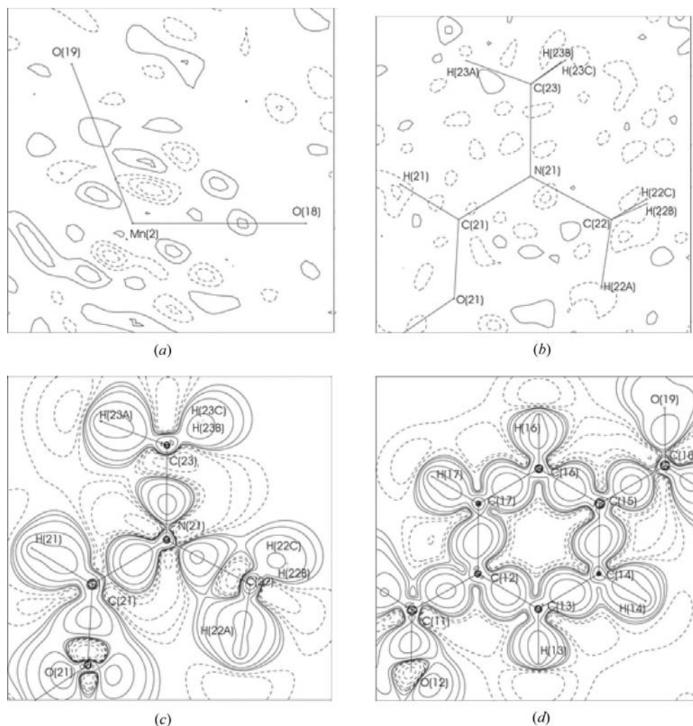
Figure 2 Residual density in the (a) Mn(2)/O(18)/O(19) plane and (b) C(21)/C(22)/C(23) plane of the DMF ligand bonded to Mn(1). (c) and (d) show the static deformation density in the C(21)/C(22)/C(23) plane of the DMF ligand bonded to Mn(1) and of a benzene ring of a BDC linker molecule, respectively. The contour level is 0.1 \text{ e \AA}^{-3} . Solid lines are positive and dashed lines are negative.
